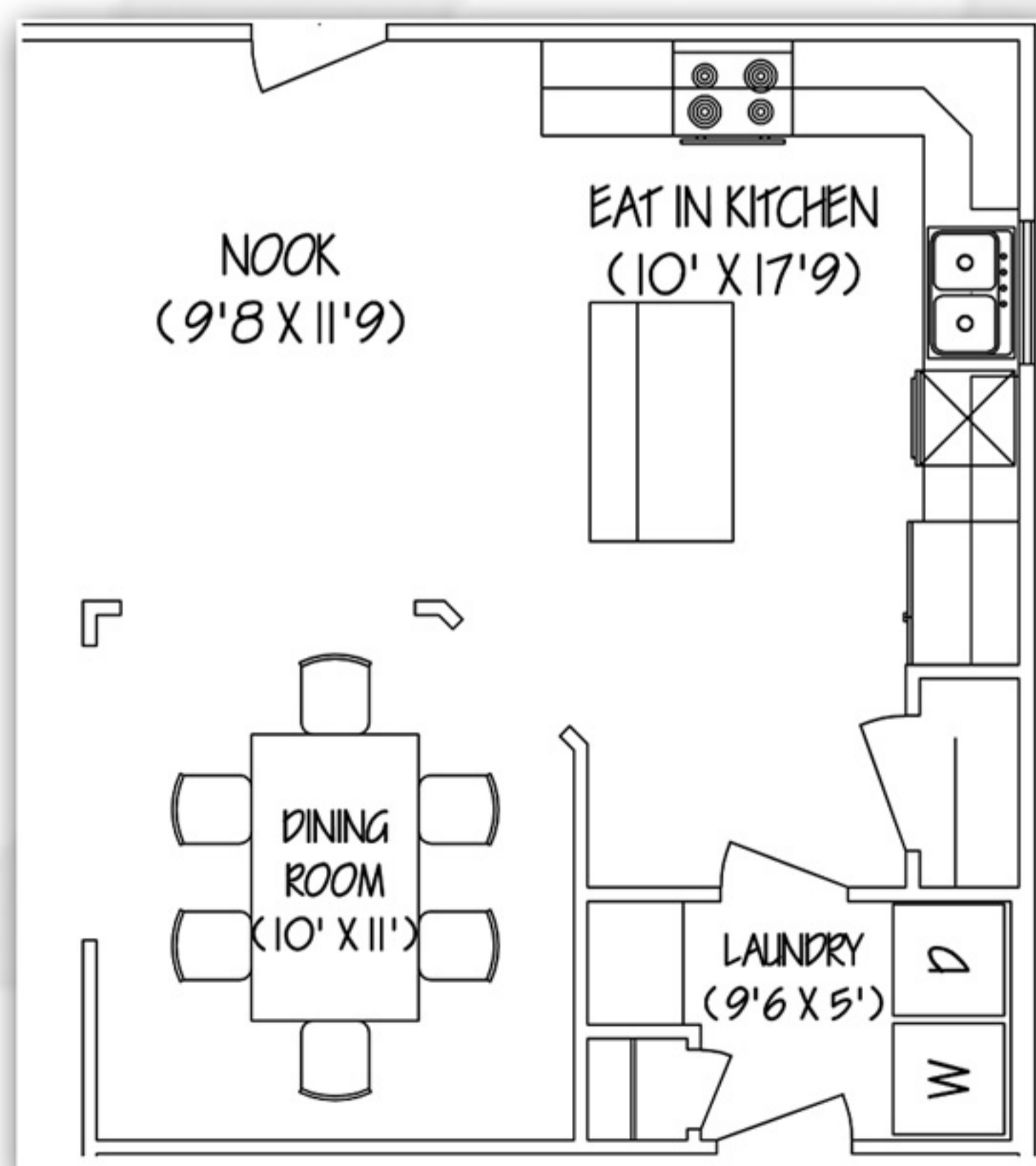
Optional Layout for Extra Dining Space
